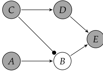
Figure 2: Preemption.
